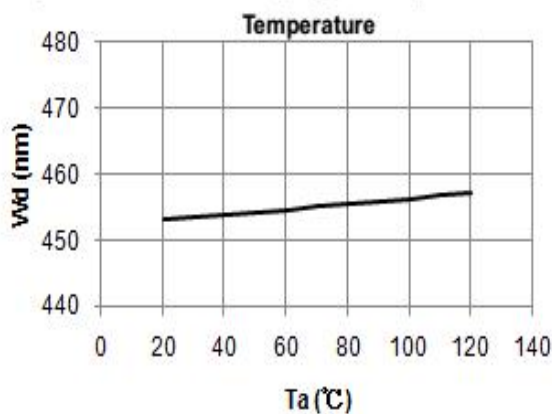
Fig.5- Dominant Wavelength (@120mA) vs. Ambient Temperature
