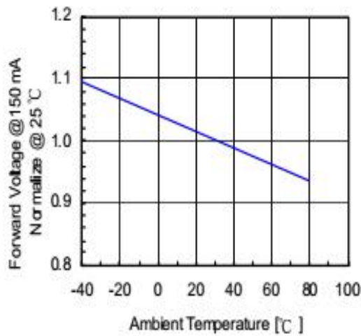
Fig 3. Forward Voltage vs. Temperature
