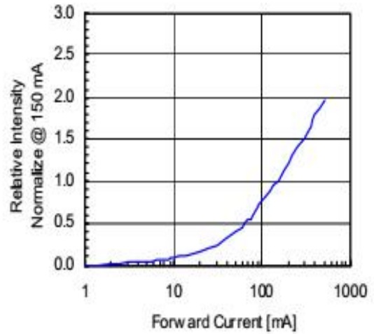
Fig 2. Relative Intensity vs. Forward Current
