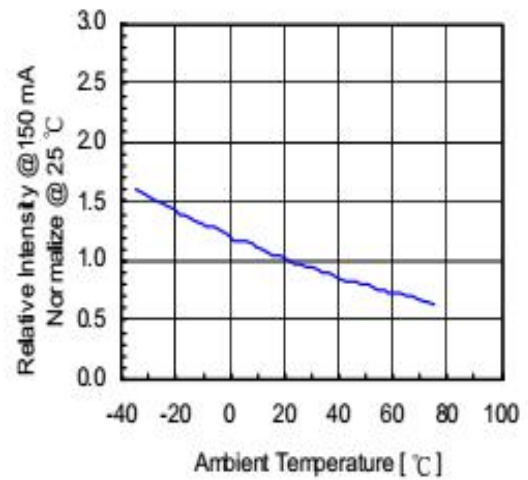
Fig 4. Relative Intensity vs. Temperature
